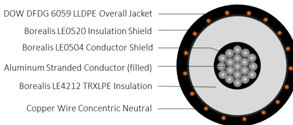
CABLE DRAWING
