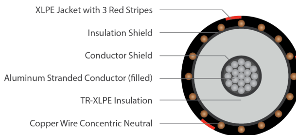
SERIES E9MWT
